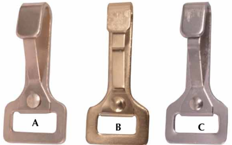
Stamped Steel Spring Snaps Brass Plated A. No. 16418 \frac{3}{4} " x 2\frac{1}{2} " B. No. 16420 1" x 2\frac{1}{2} " Nickel Plated C. No. 16421 1" x 2\frac{1}{2} "
