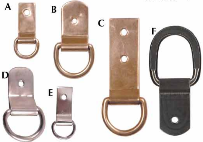
Solid Brass Clip & Dee A. No. 16637B dee - 5/8" clip - 1 1/2" overall length - 2 1/4" B. No. 16630-2 dee - 1" clip - 2" overall length - 3" C. No. 16630B dee - 1" clip - 3" overall length - 4" Nickel Plated Clip & Dee D. No. 16630 dee - 1" clip - 2" overall length - 3" E. No. 16637 dee - 1/2" clip - 1 1/2" overall length - 2" Stainless Steel Clip & Dee F. No. 16630-3 dee - 1 7/8" clip - 1 3/4" overall length - 3 1/8"
